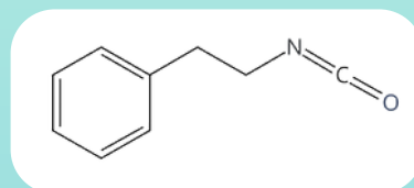
2-Phenylethylisocyanate CAS 1943-82-4
